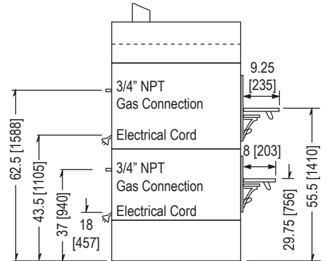
STACKED OVEN SIDE VIEW
