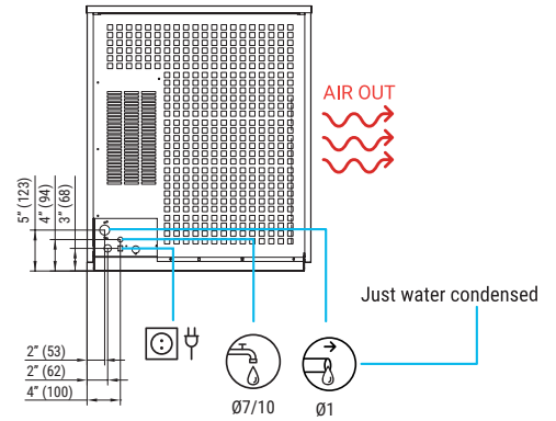
REAR VIEW VISTA TRASERA
