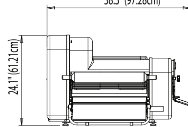
Floor View
